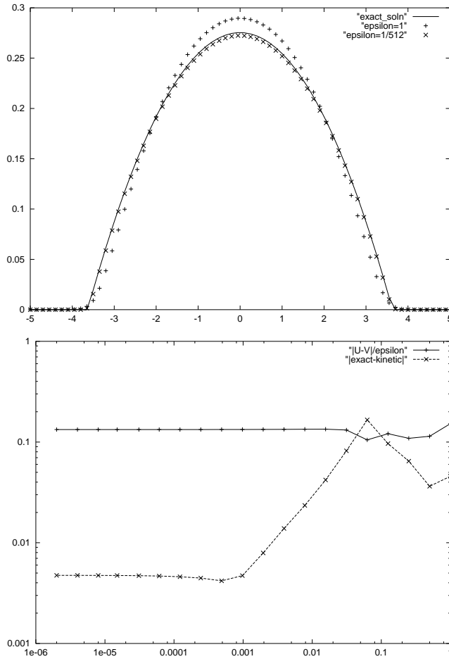
Fig. 3. Results for (18)–(34) on (5)–(6) with Barenblatt’s solution.
